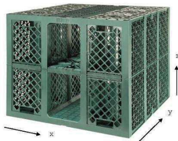
Figure 1 a- Module Rigofill inspect
